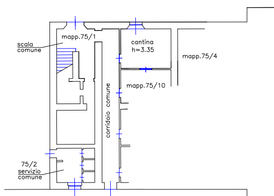
PIANO TERRA
